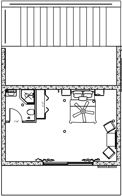
SERENITY HEIGHTS Concept first floor plan
