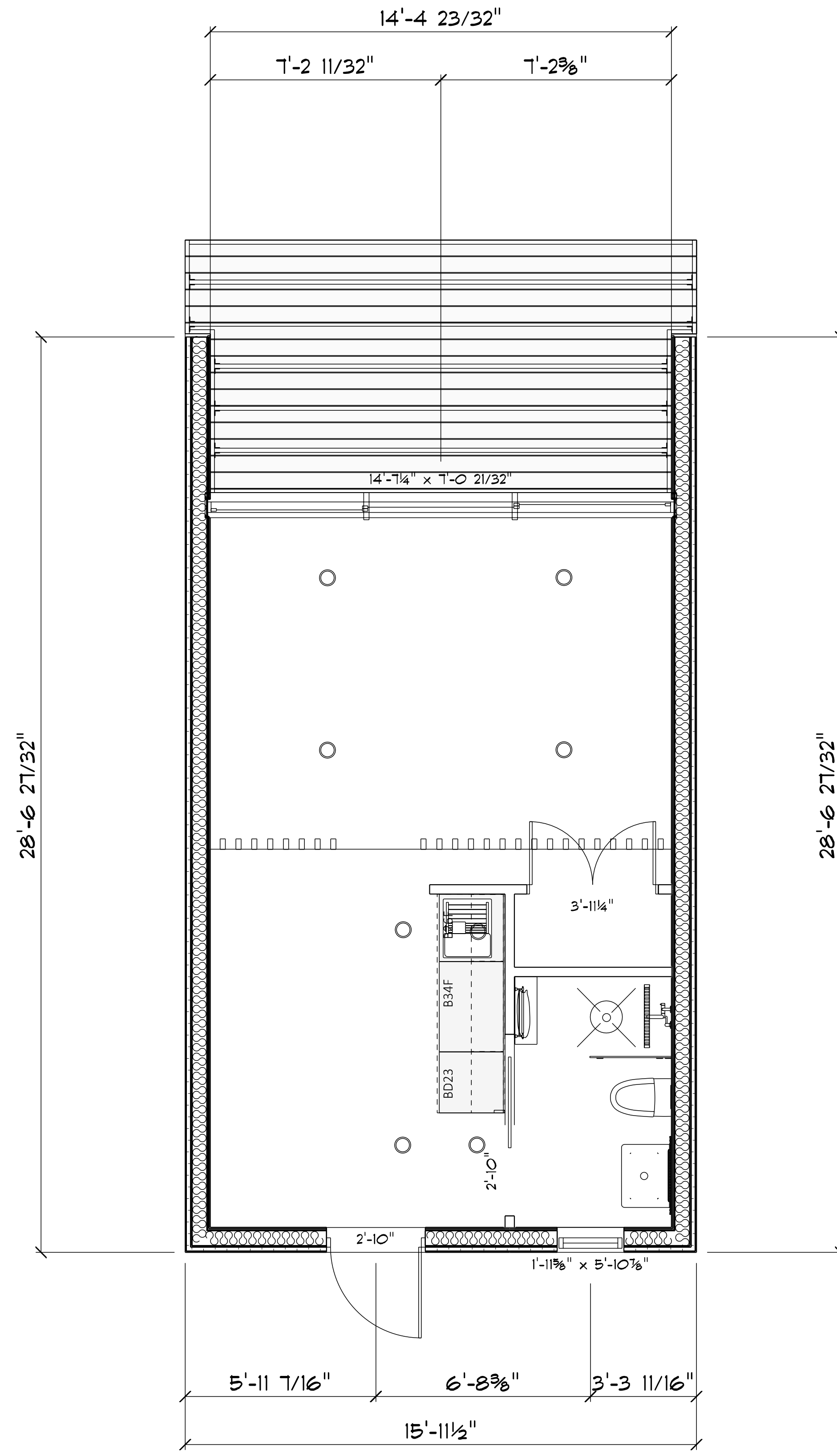
GROUND FLOOR SCALE: 3/8" = 1'-0"
