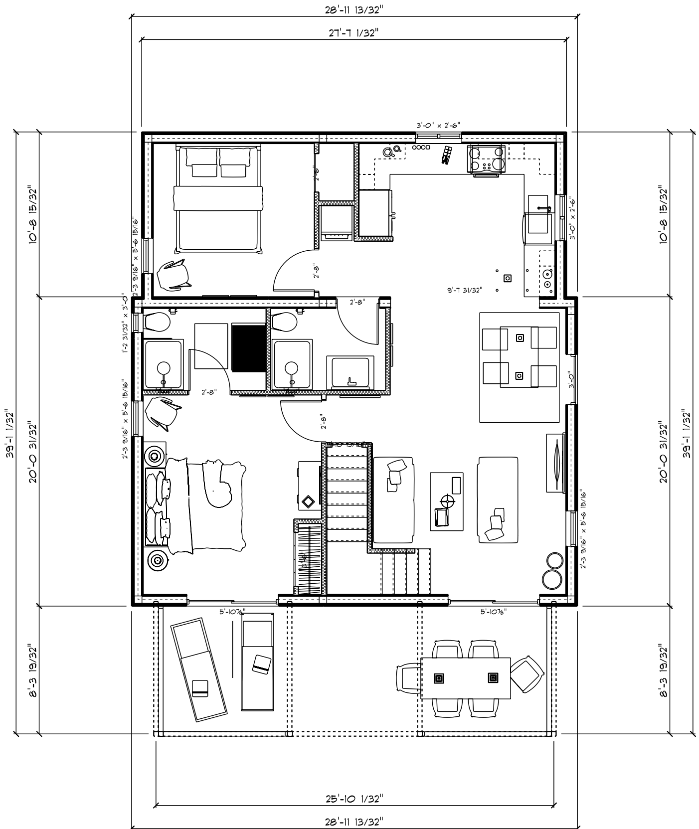
The Palm Cottage ground floor
